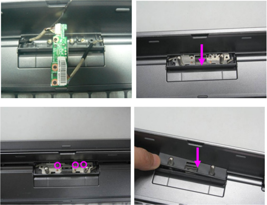
Figure 3-46. Connector Board
