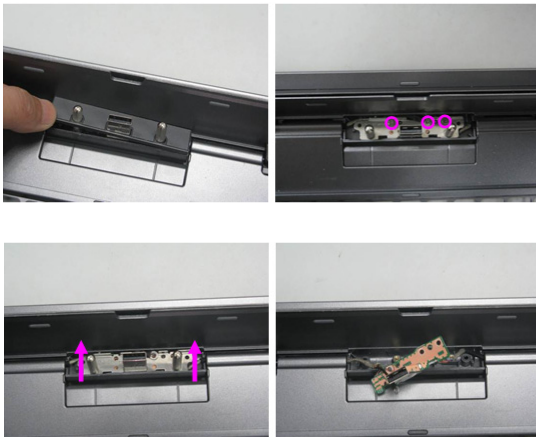
Figure 3-27. Connector Board
