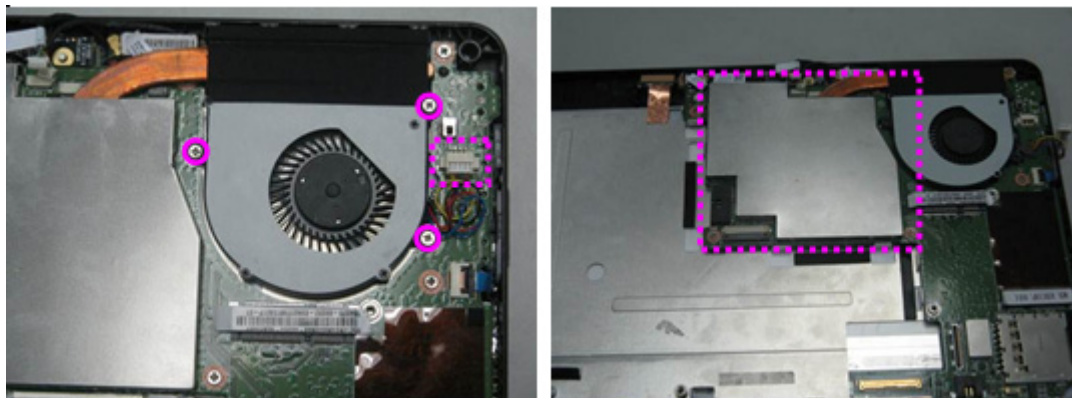
Figure 3-12. Thermal Module
