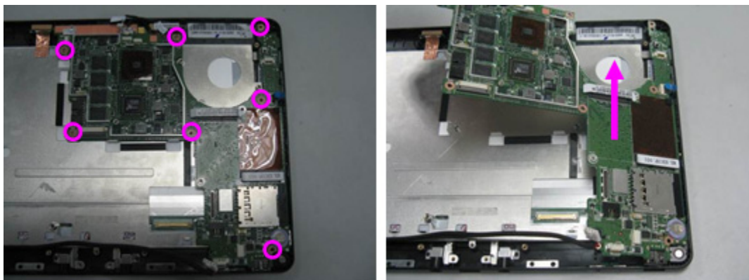
Figure 3-16. Motherboard Module
