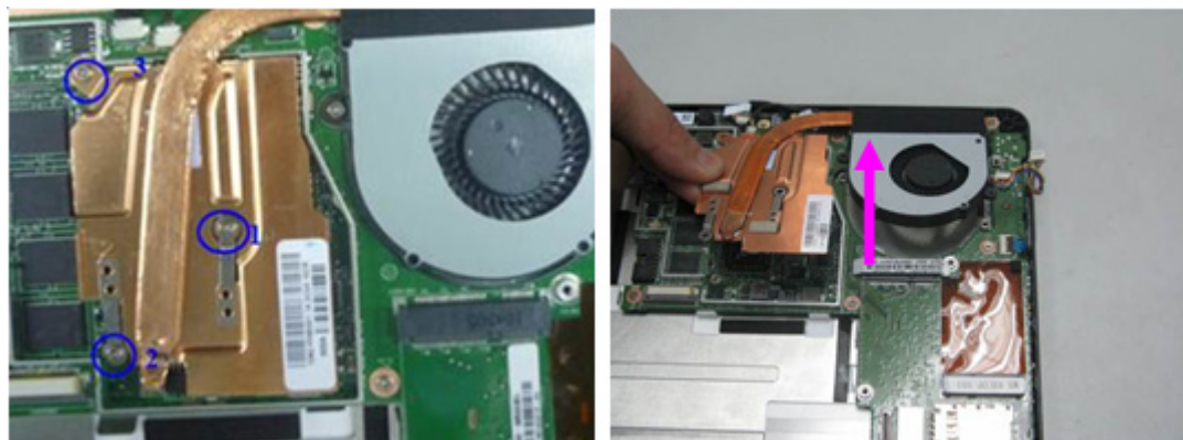
Figure 3-13. Thermal Module
