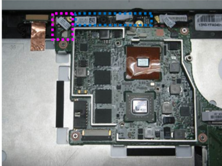
Figure 3-33. Camera Module
