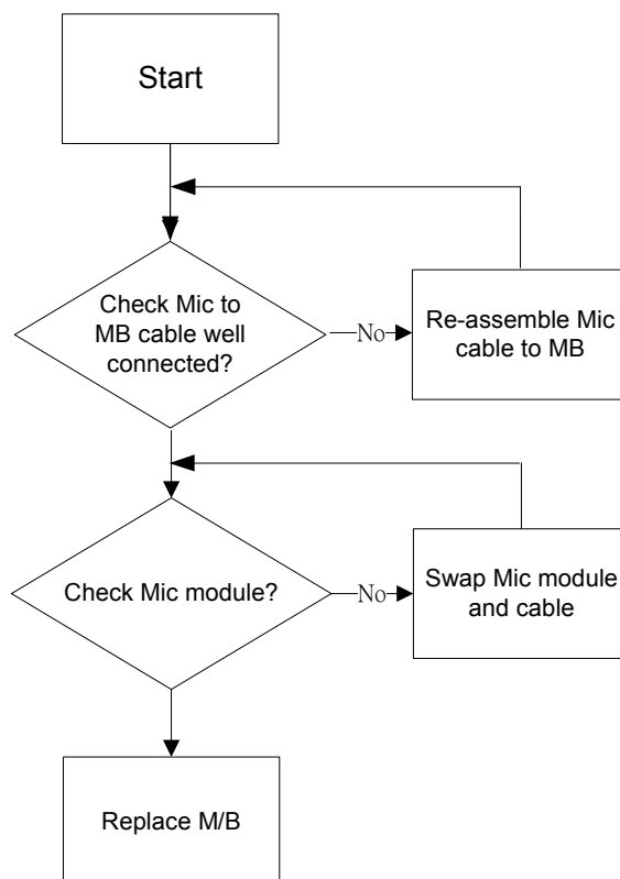
Figure 4-6. Microphone Failure
