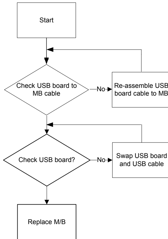
Figure 4-7. USB Failure
