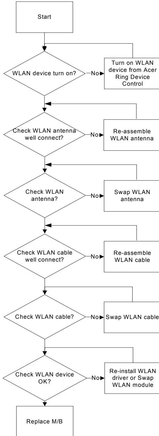
Figure 4-8. WLAN Failure
