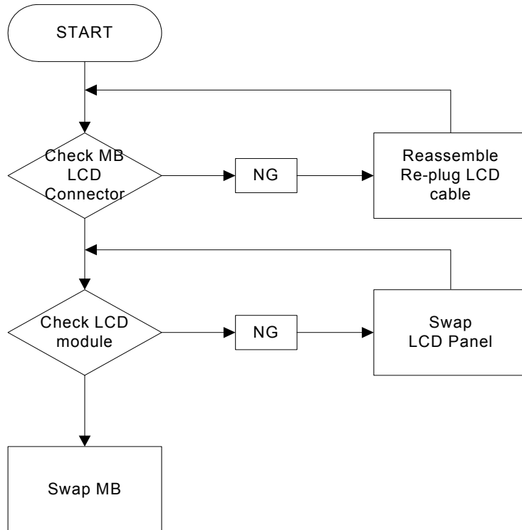
Figure 4-3. LCD Failure
