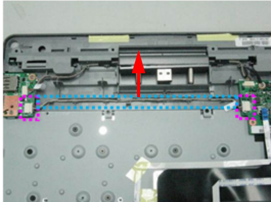
Figure 3-21. USB Cable
