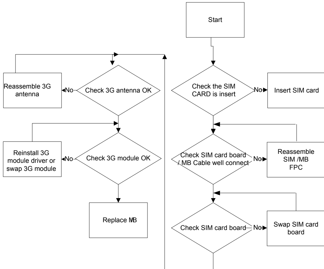
Figure 4-10. 3G Failure
