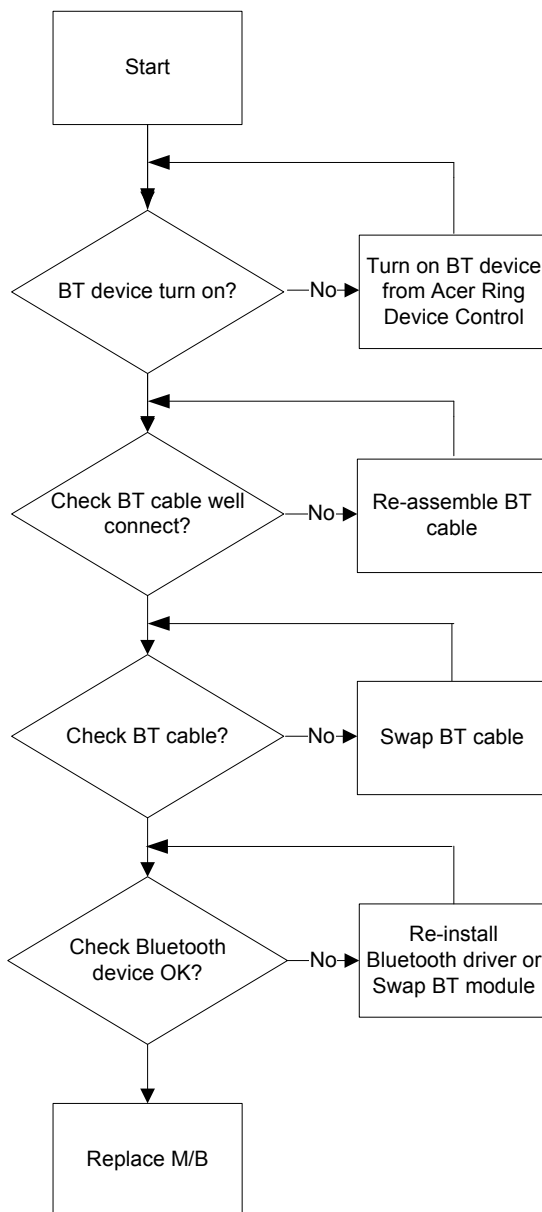
Figure 4-9. Bluetooth Failure
