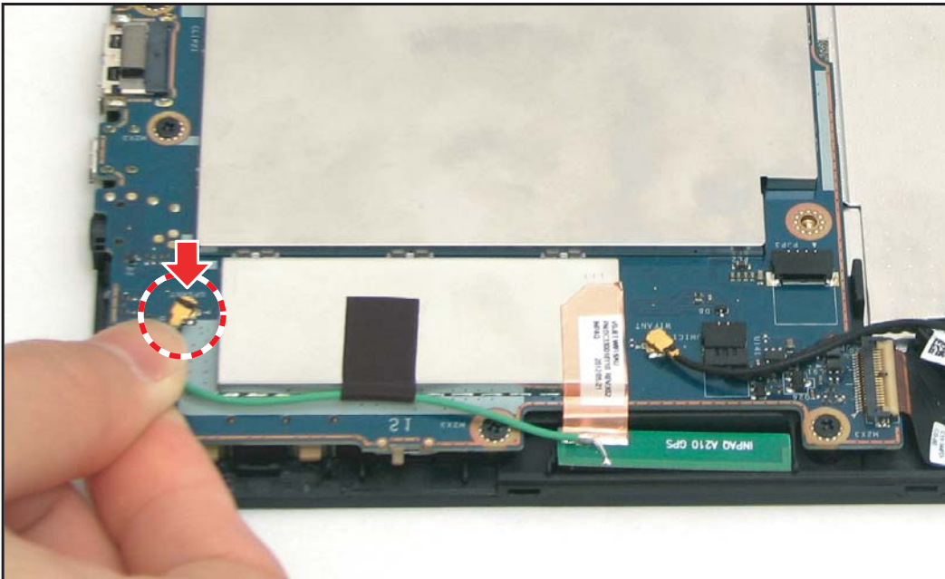
Figure 5-78. Installing the GPS Antenna (4 of 4)
