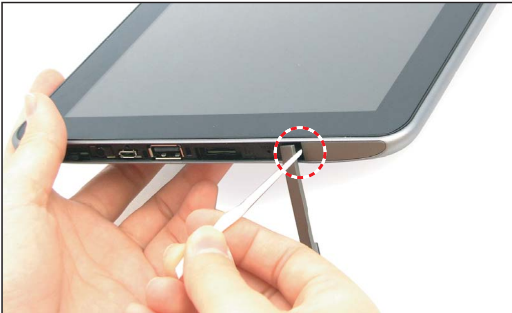
Figure 5-10. Unlocking the Left IO Cover Latches (3 of 4)
