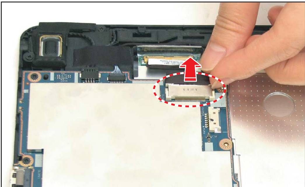
Figure 5-56. Disconnecting the LVDS Cable (1 of 2)
