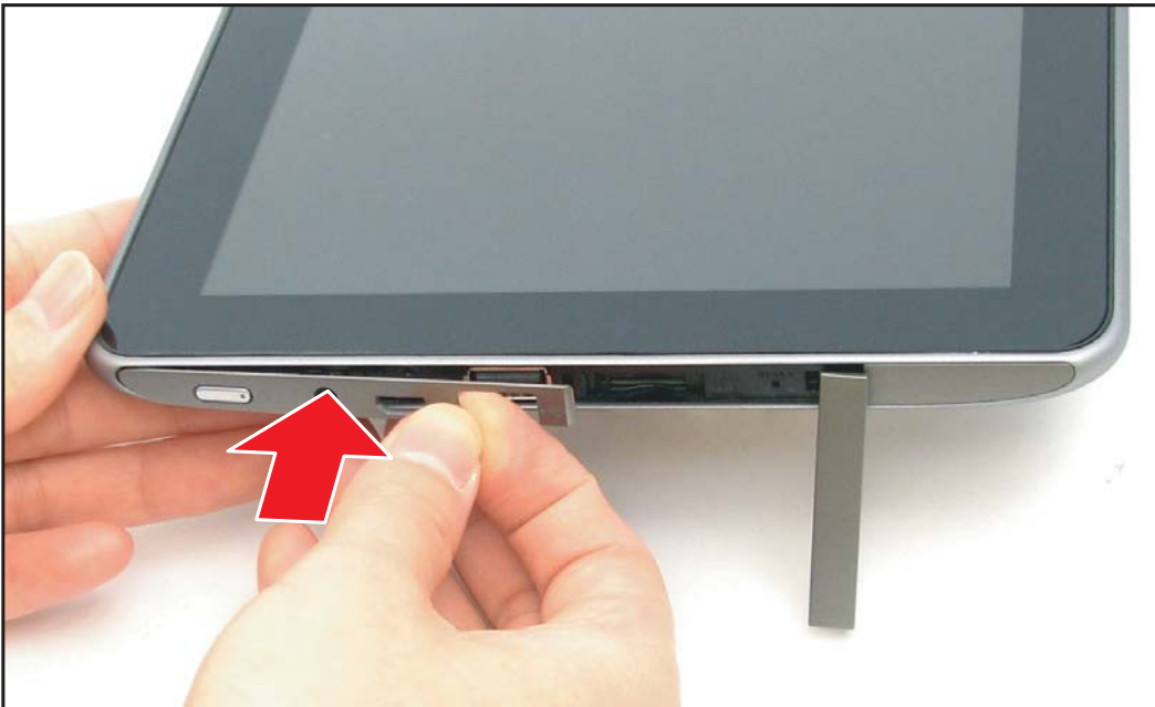
Figure 5-26. Installing the Left IO Cover (2 of 2)
