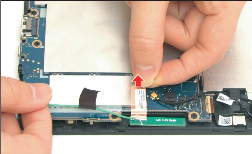
Figure 5-73. Removing the Antenna Metallic Tape
