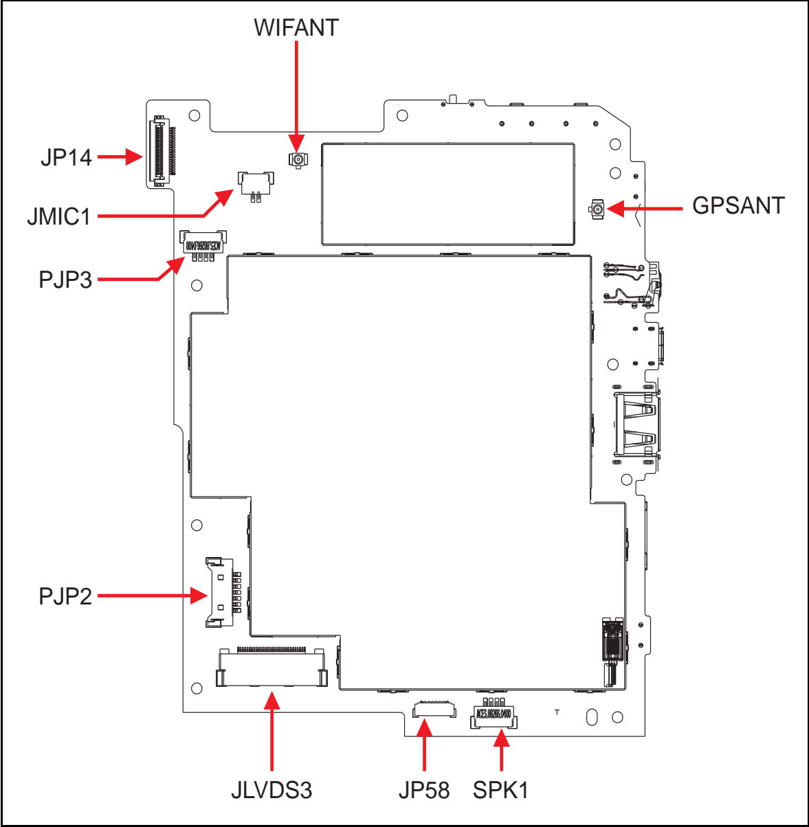
Figure 3-2. Mainboard Bottom
