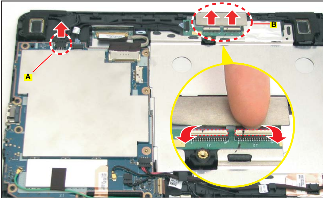
Figure 5-42. Disconnecting the Speakers and Touch Panel Cables
