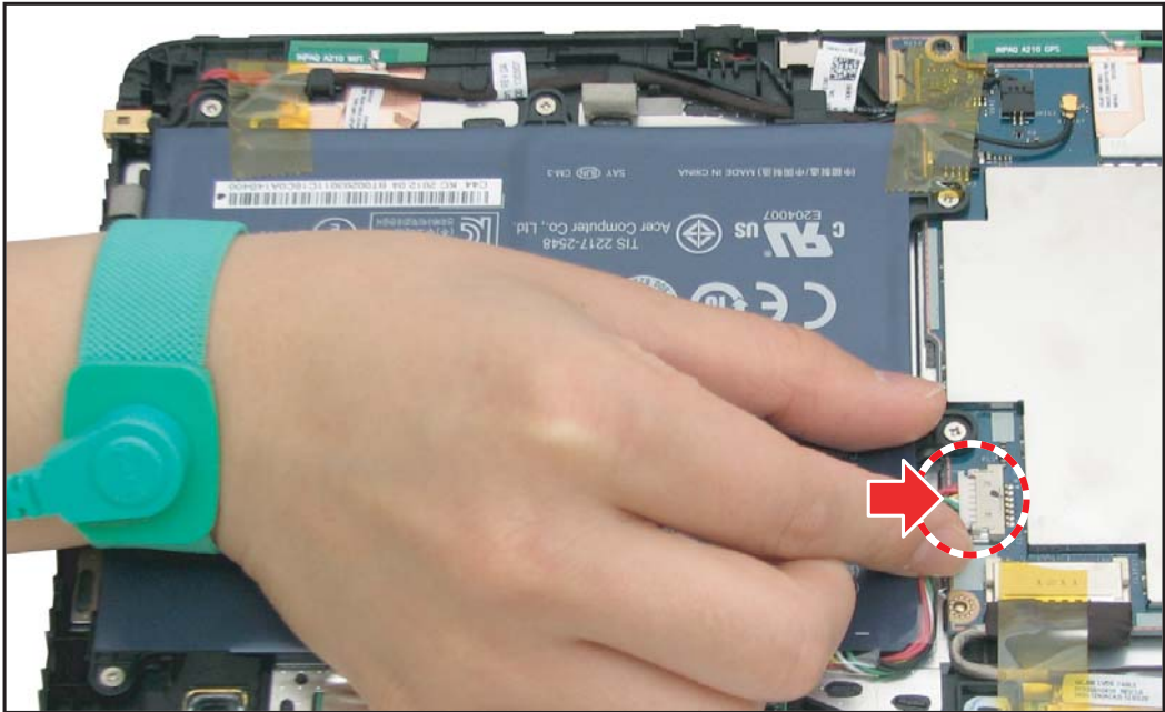
Figure 5-33. Connecting the Battery Cable
