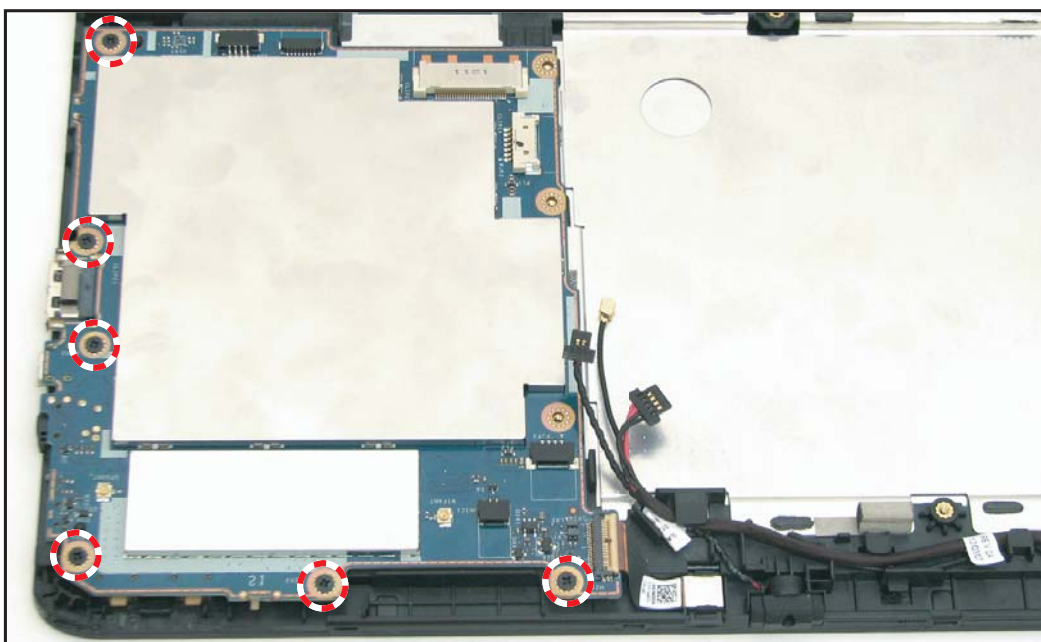
Figure 5-85. Securing the Mainboard Screws
