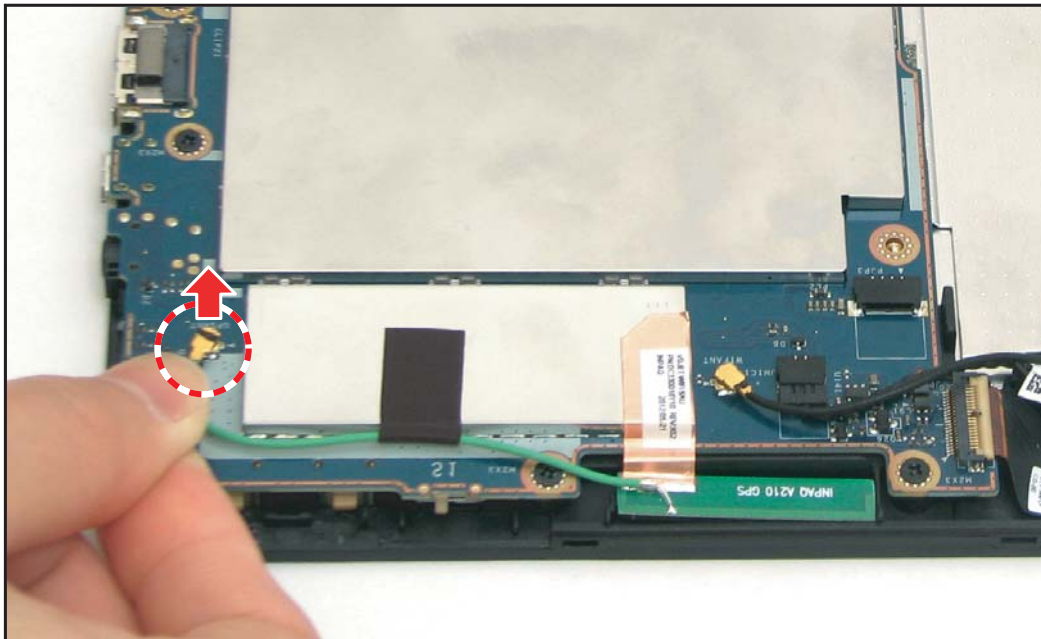
Figure 5-71. Disconnecting the GPS Antenna
