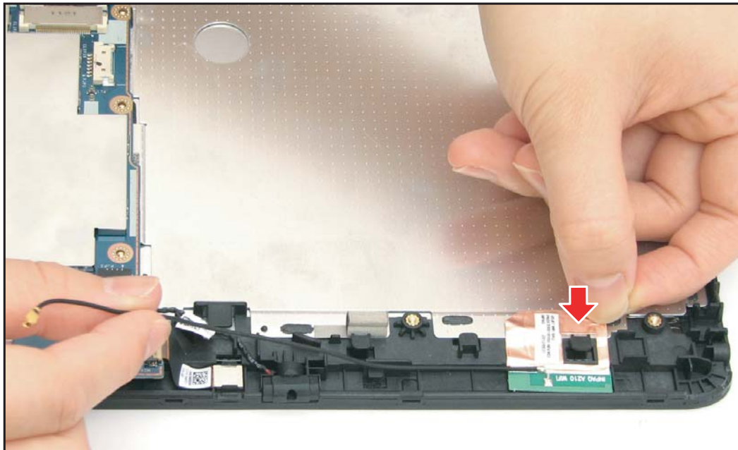
Figure 5-69. Installing the WLAN Antenna (2 of 3)
