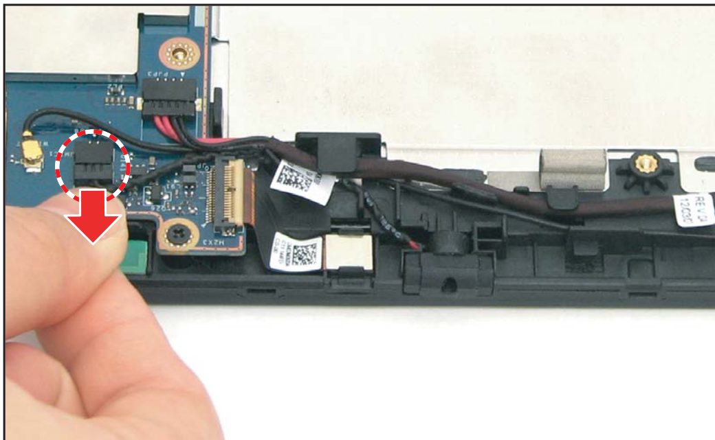
Figure 5-61. Disconnecting the Microphone Connector
