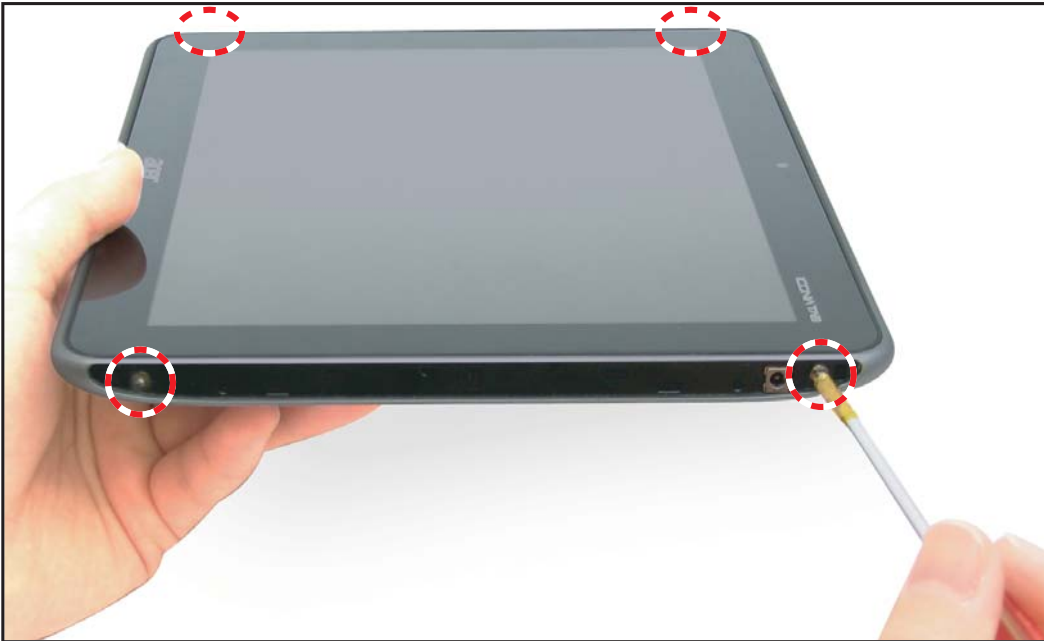
Figure 5-23. Installing the Lower Case (4 of 4)
