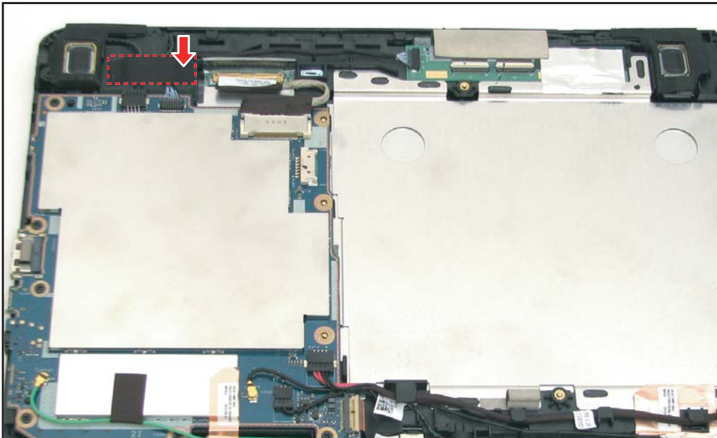
Figure 5-47. Attaching the Mylar
