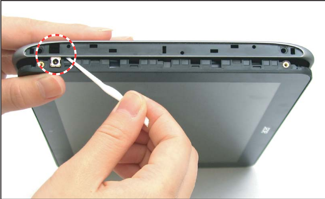
Figure 5-21. Installing the Lower Case (2 of 4)
