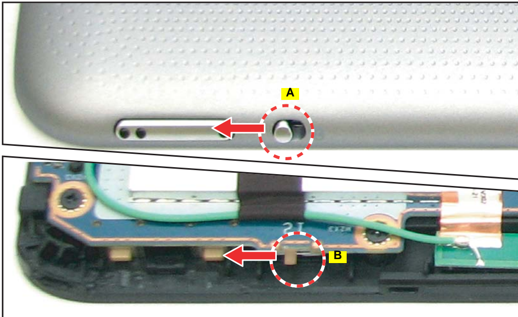
Figure 5-19. Checking the Lock Key Position
