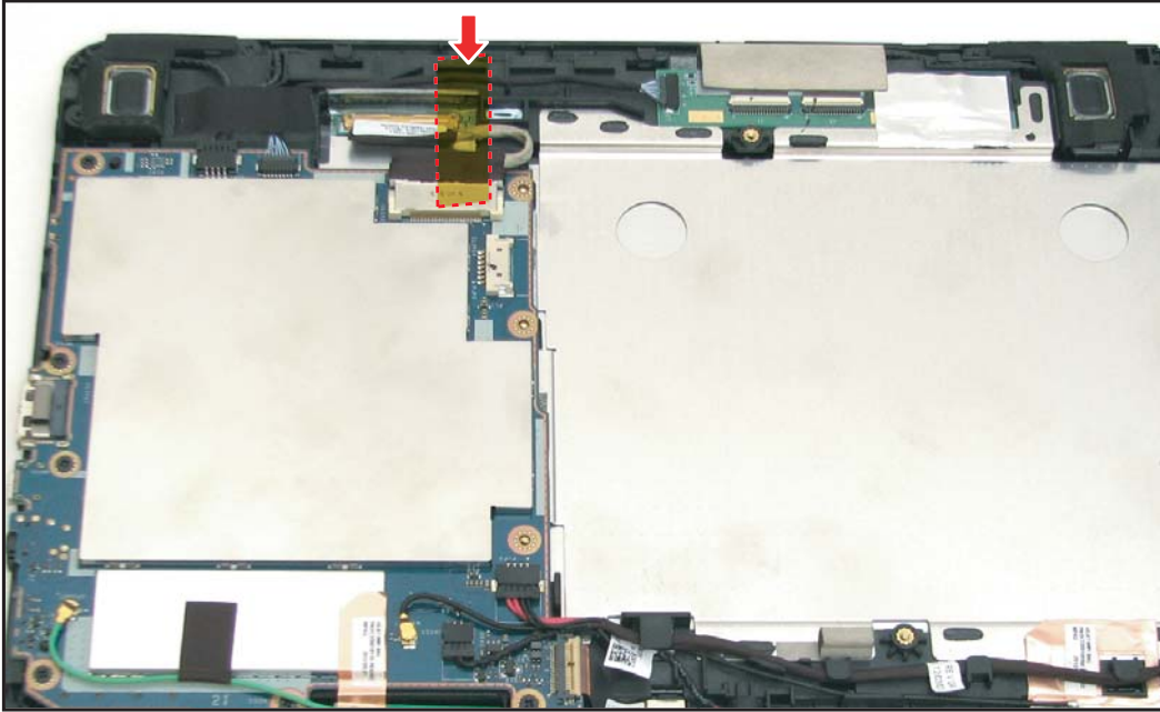
Figure 5-60. Attaching the LVDS Cable Protective Tape
