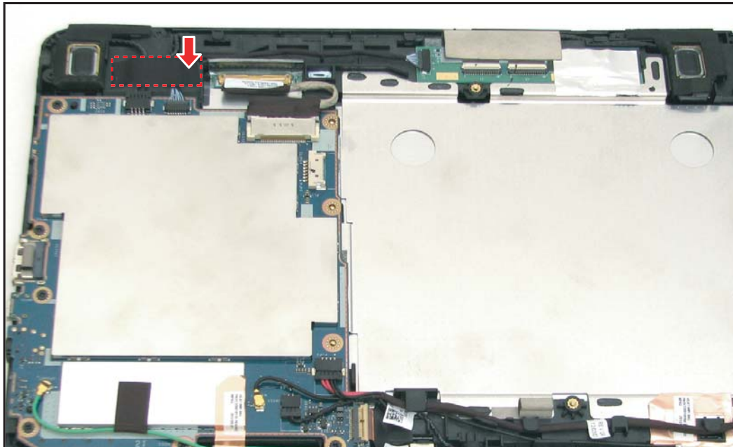
Figure 5-53. Attaching the Mylar
