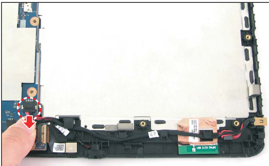
Figure 5-35. Disconnecting the DC-In Cable
