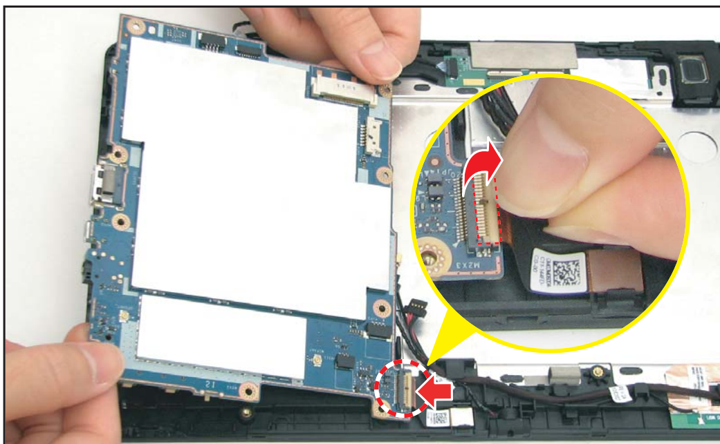
Figure 5-84. Connecting the Camera Cable
