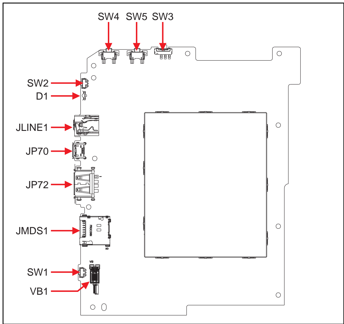
Figure 3-1. Mainboard Top
