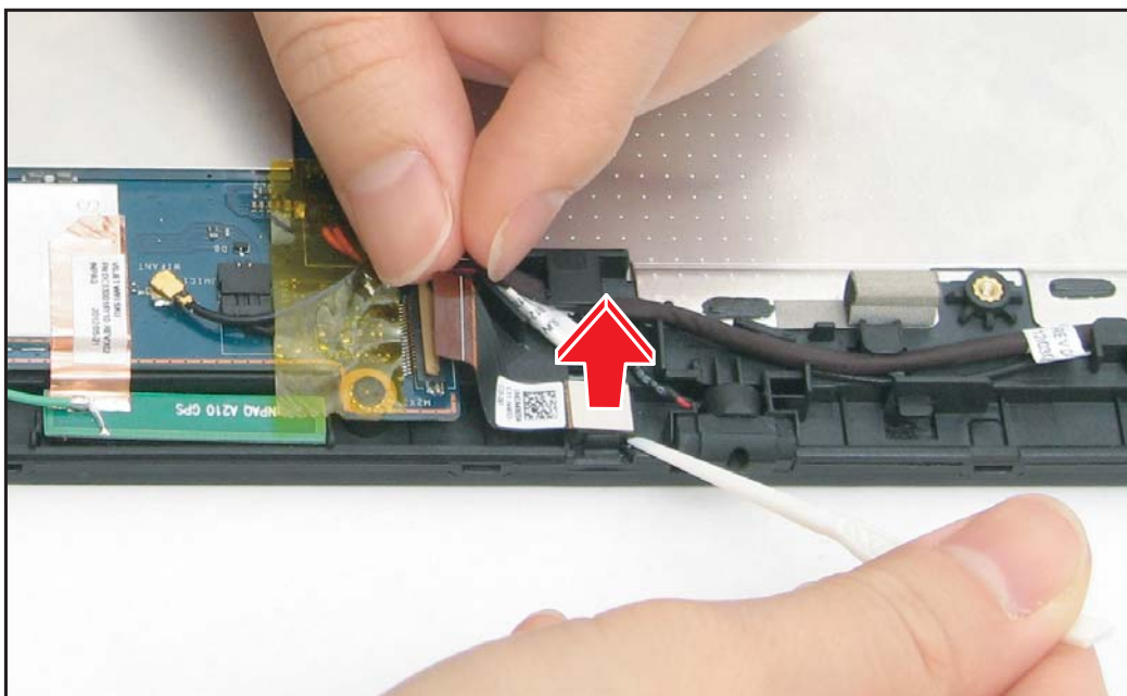
Figure 5-88. Removing the Front Camera
