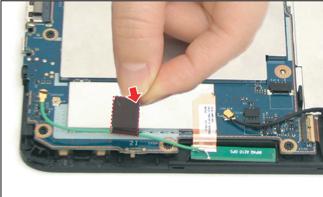
Figure 5-77. Installing the GPS Antenna (3 of 4)
