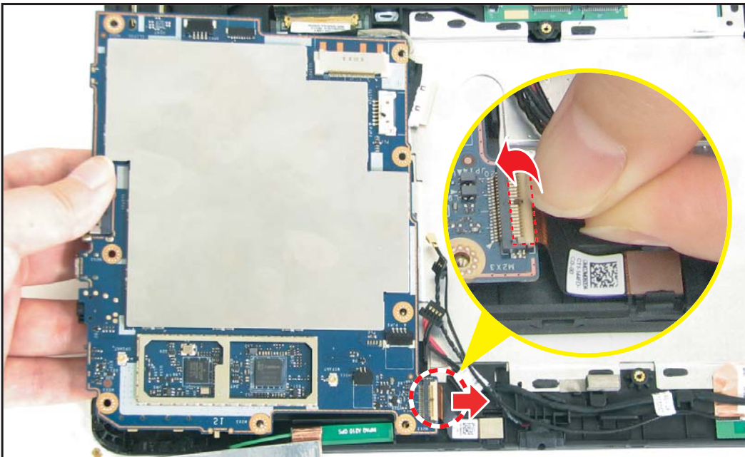
Figure 5-83. Removing the Mainboard
