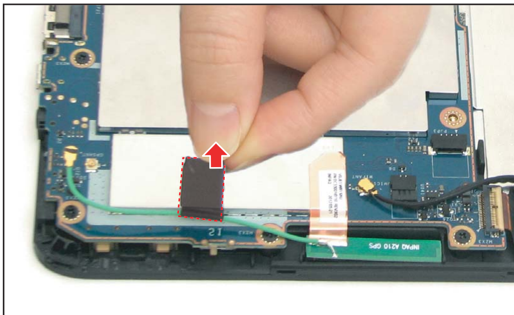
Figure 5-72. Removing the Mylar
