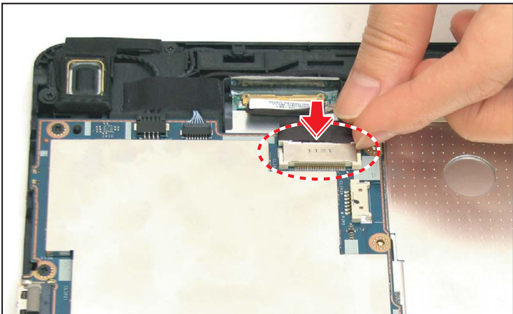
Figure 5-59. Connecting the LVDS Cable (2 of 2)
