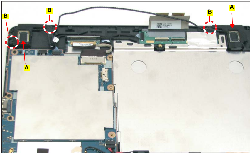
Figure 5-44. Installing the Speakers
