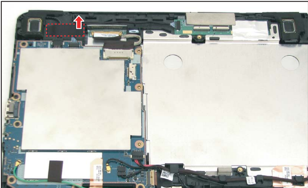
Figure 5-41. Removing the Mylar
