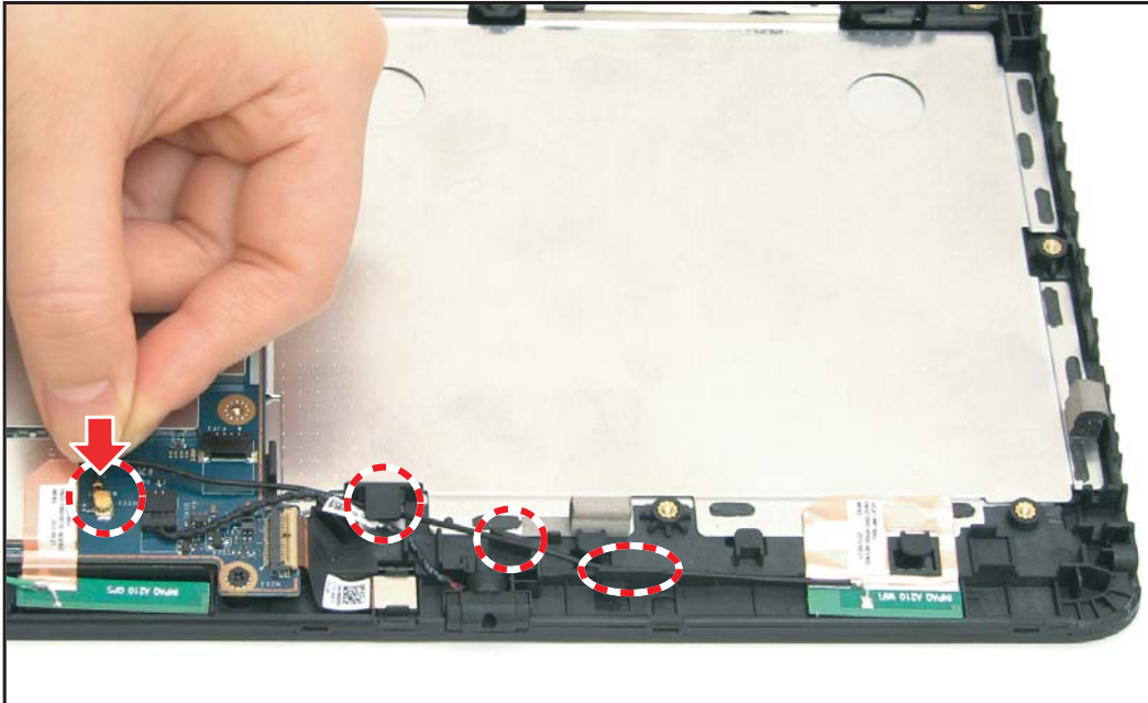
Figure 5-70. Installing the WLAN Antenna (3 of 3)
