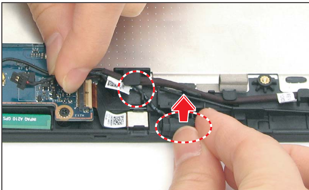
Figure 5-62. Removing the Microphone
