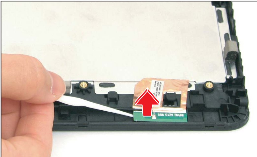
Figure 5-67. Removing the WLAN Antenna
