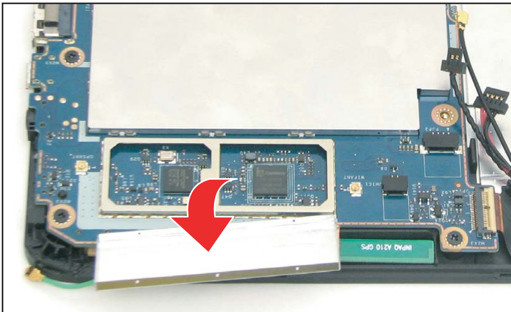
Figure 5-81. Removing the Circuit Cover (2 of 2)
