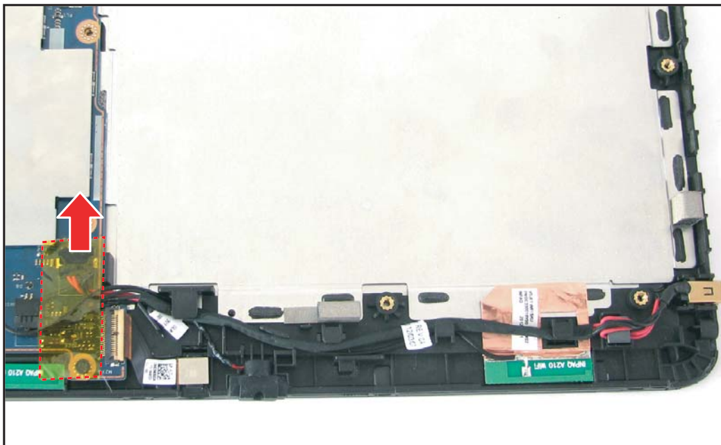
Figure 5-34. Removing the Protective Tape
