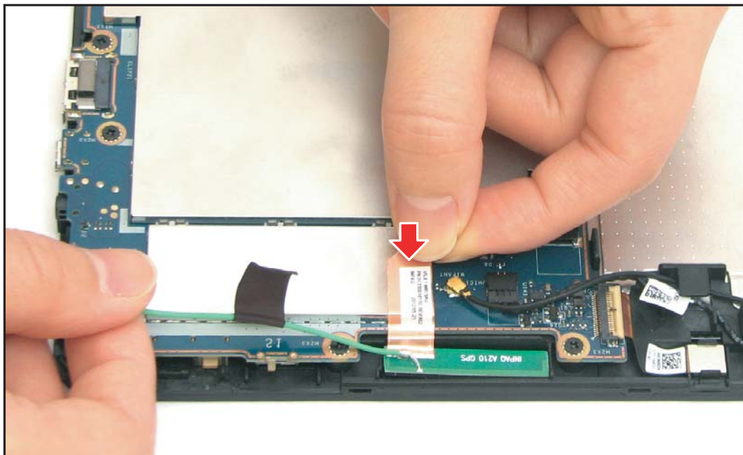
Figure 5-76. Installing the GPS Antenna (2 of 4)
