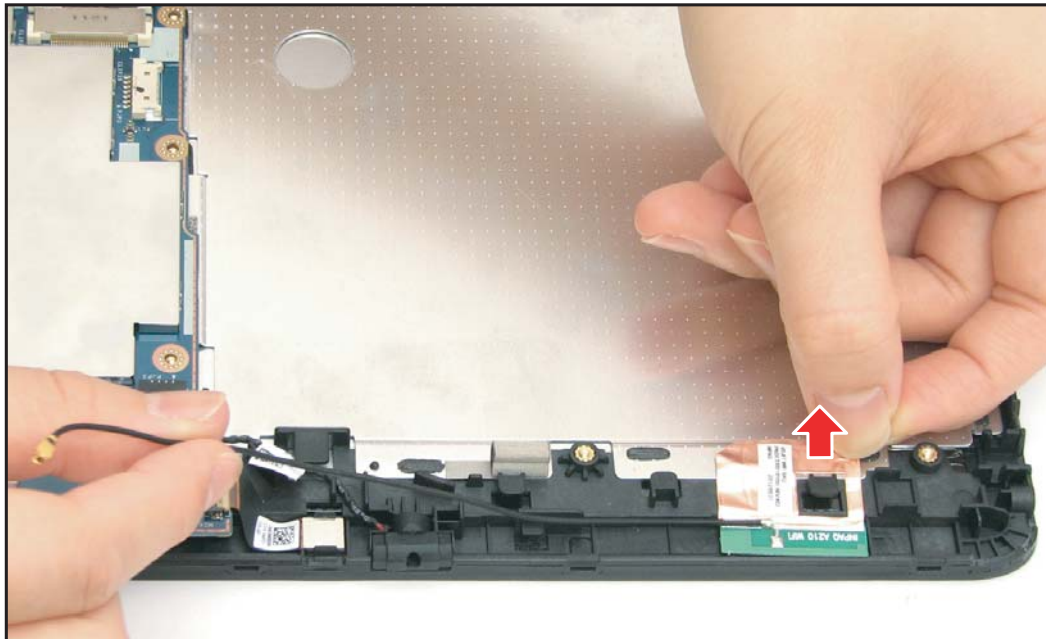
Figure 5-66. Removing the Metallic Tape
