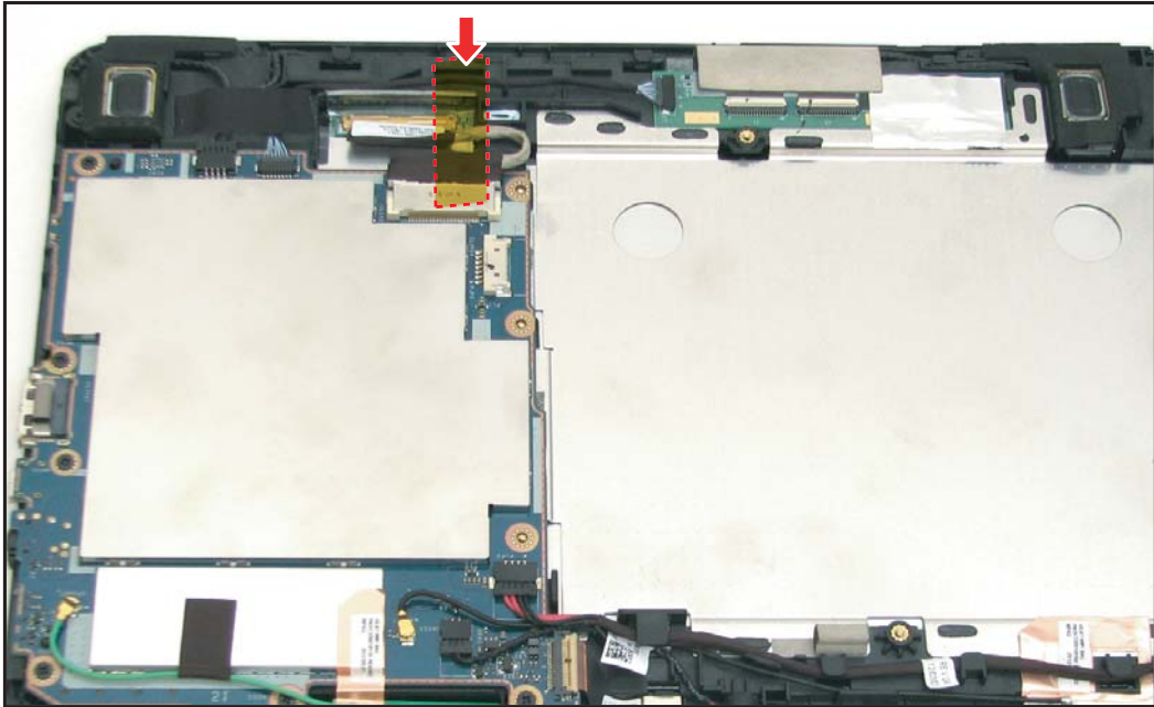
Figure 5-54. Attaching the LVDS Protective Tape
