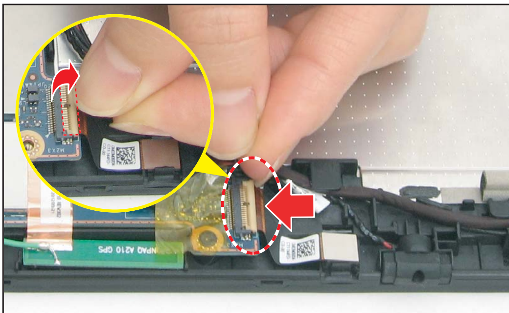
Figure 5-90. Connecting the Camera Cable
