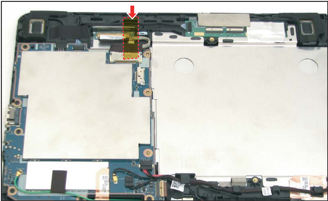
Figure 5-48. Attaching the LVDS Protective Tape
