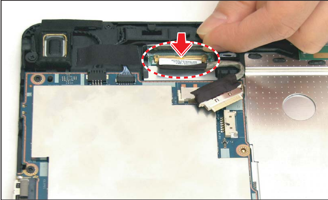
Figure 5-57. Disconnecting the LVDS Cable (2 of 2)
