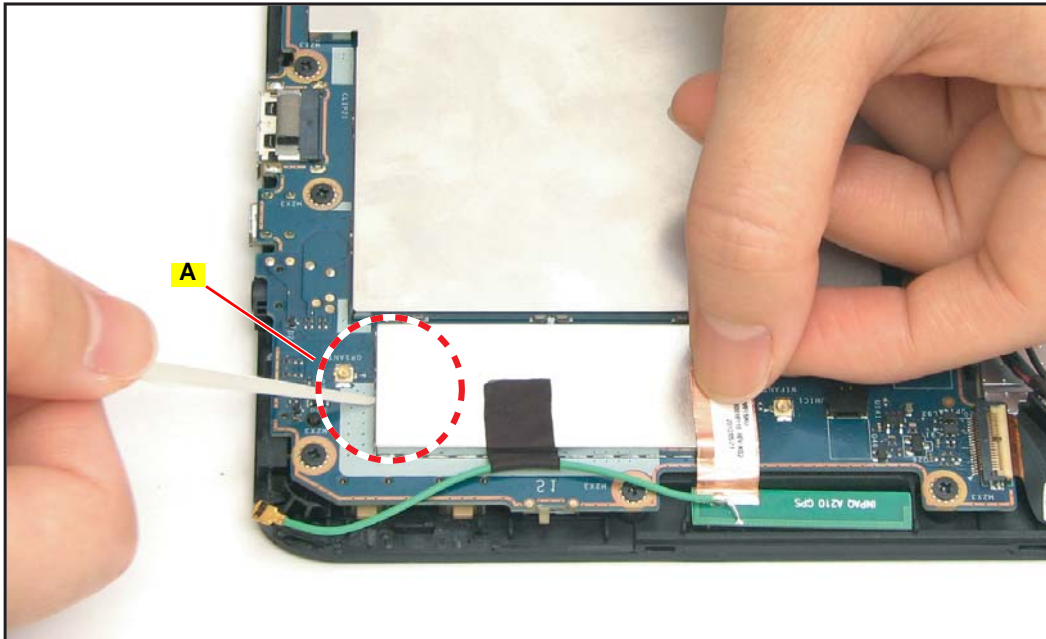
Figure 5-80. Removing the Circuit Cover (1 of 2)
