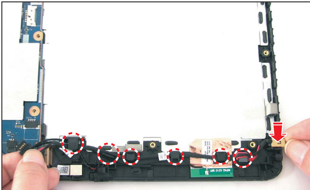
Figure 5-37. Installing the DC-In Cable (1 of 3)
