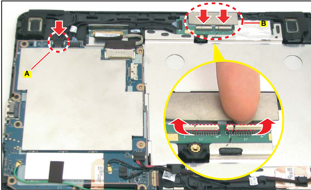
Figure 5-46. Connecting the Cable Connectors
