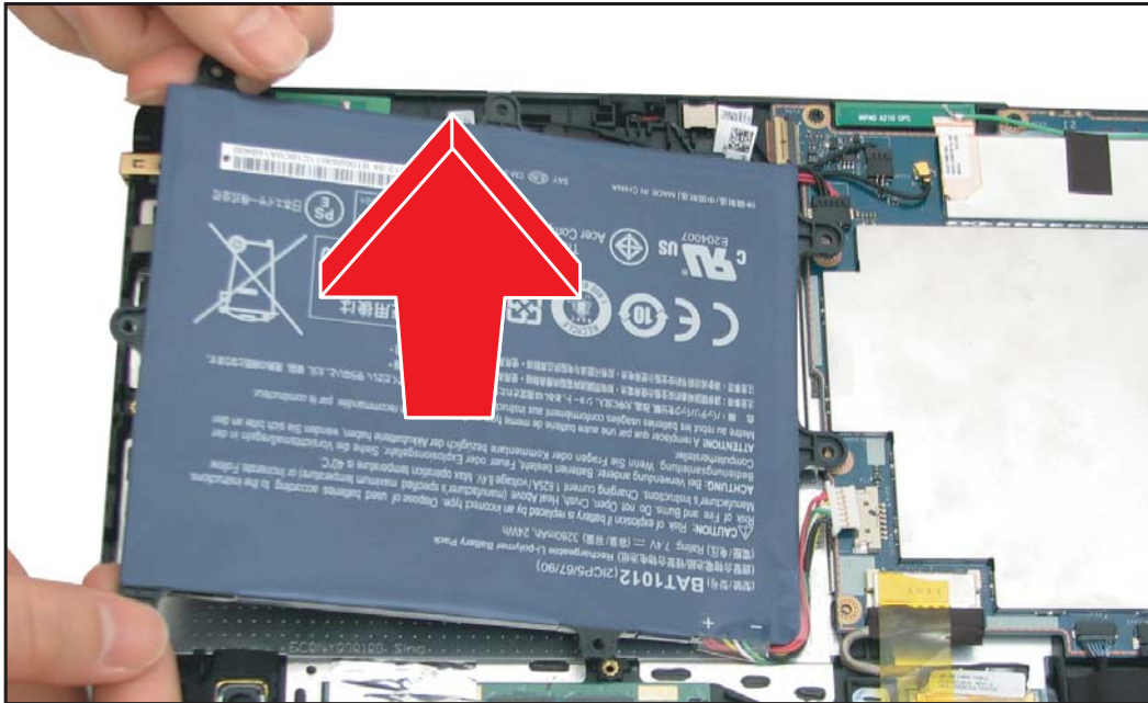
Figure 5-30. Removing the Battery
