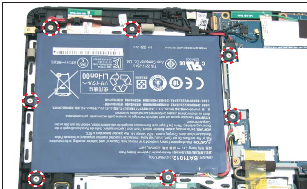
Figure 5-32. Attaching the Battery Screws
