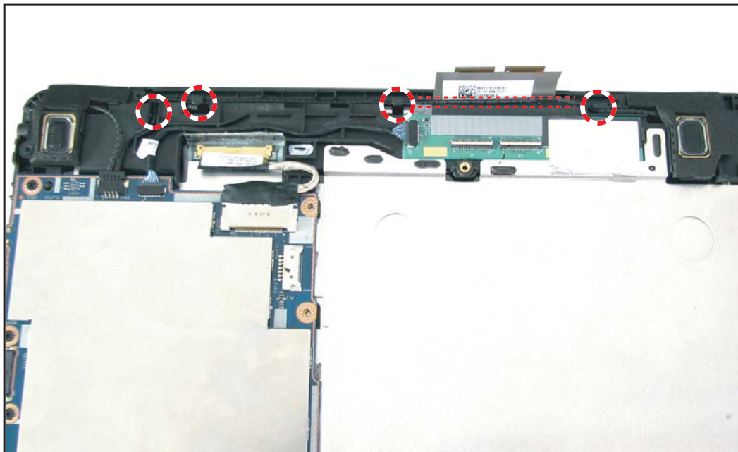
Figure 5-45. Routing the Speakers Cable
