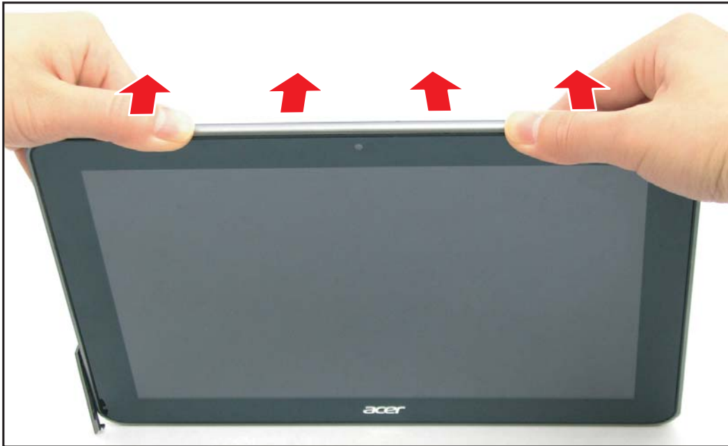
Figure 5-15. Releasing the Side Latches (1 of 4)
