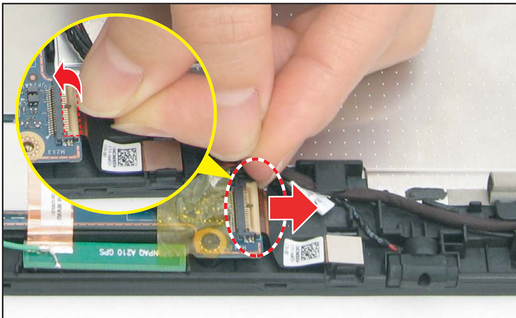
Figure 5-87. Disconnecting the Camera Cable
