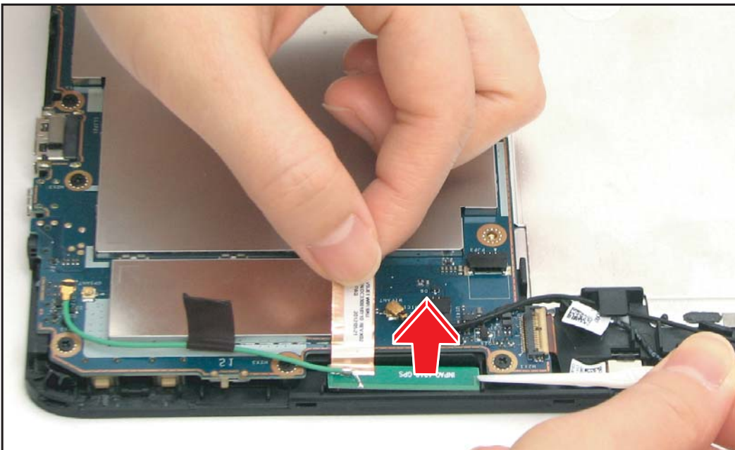
Figure 5-74. Removing the GPS Antenna
