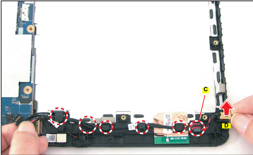
Figure 5-36. Removing the DC-In Cable
