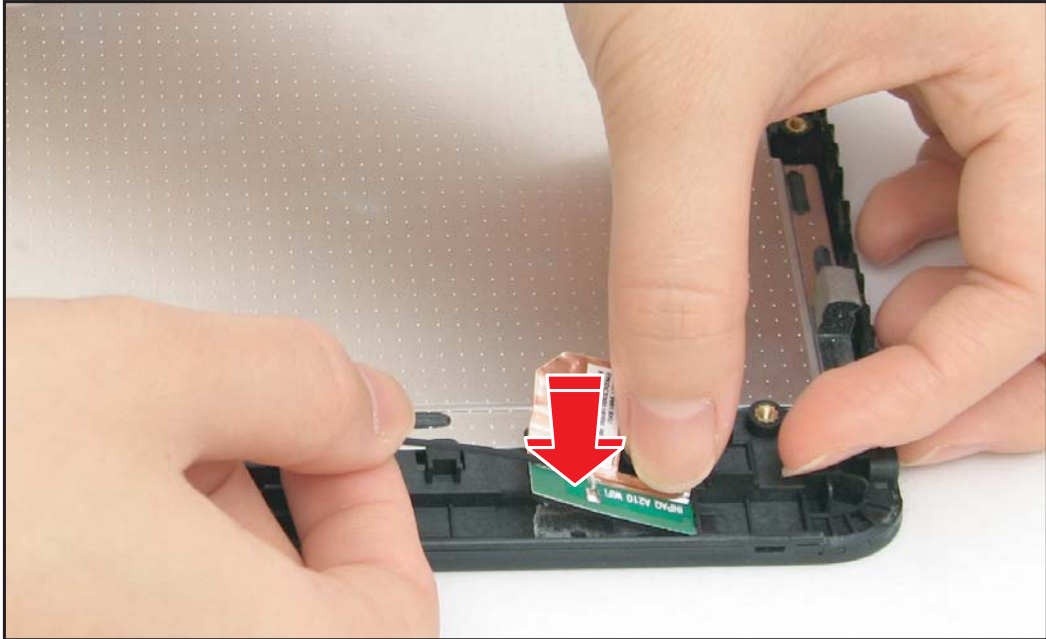
Figure 5-68. Installing the WLAN Antenna (1 of 3)
