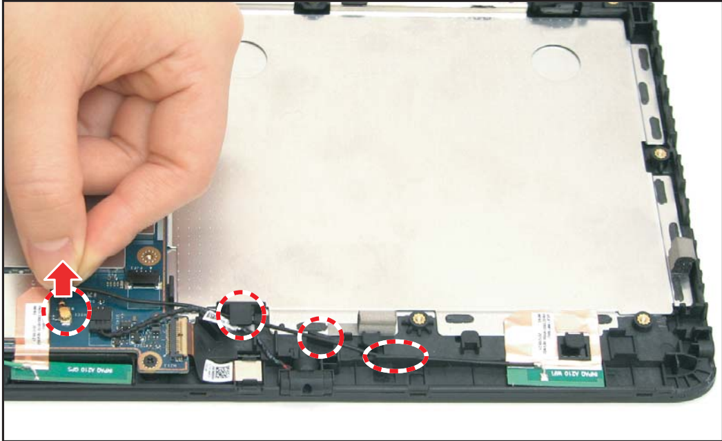
Figure 5-65. Disconnecting the WLAN Antenna
