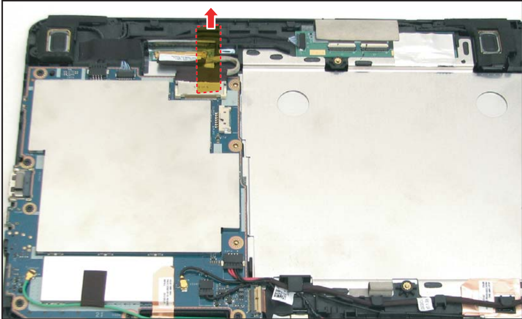
Figure 5-49. Removing the LVDS Protective Tape
