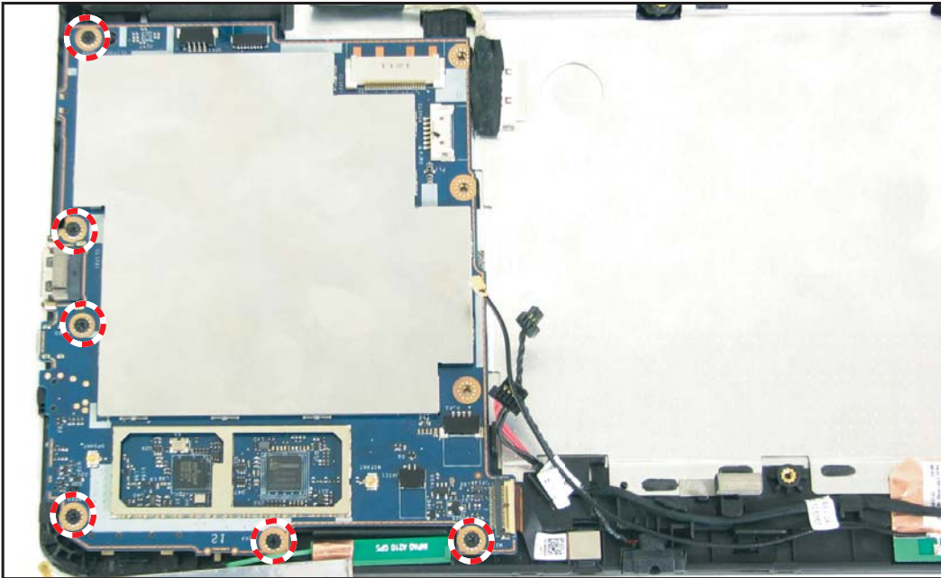
Figure 5-82. Removing the Mainboard Screws
