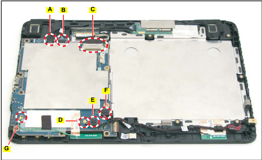
Figure 5-86. Connecting the Cables to the Mainboard
