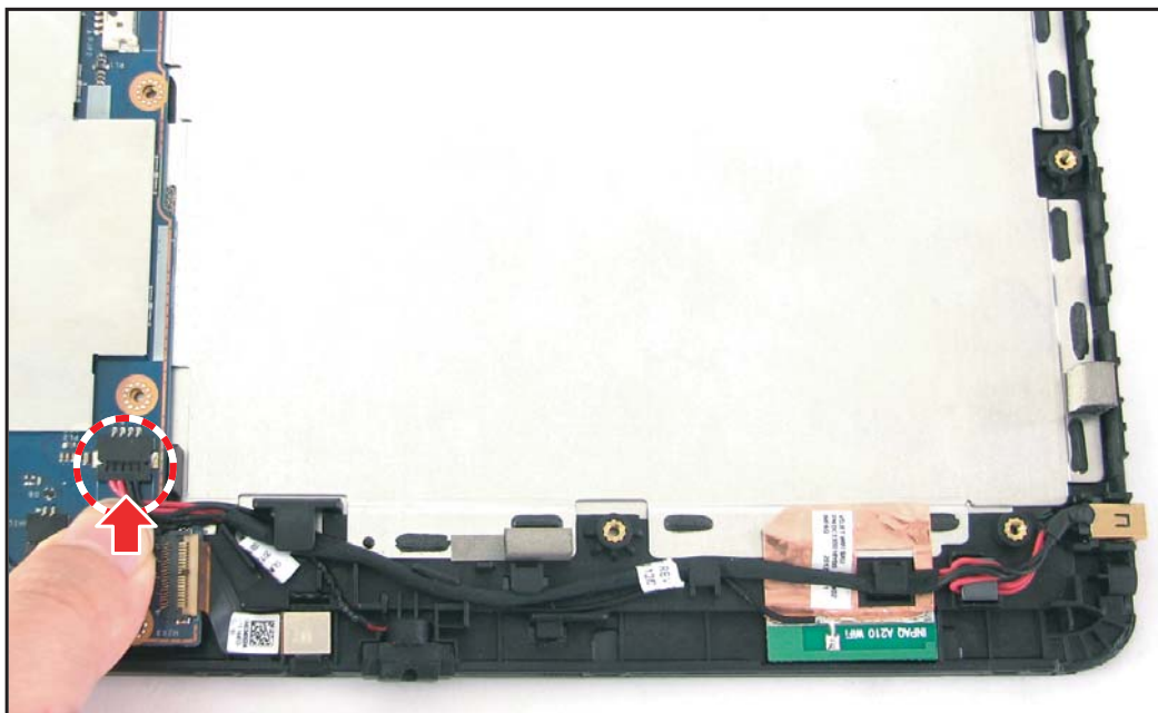
Figure 5-38. Installing the DC-In Cable (2 of 3)
