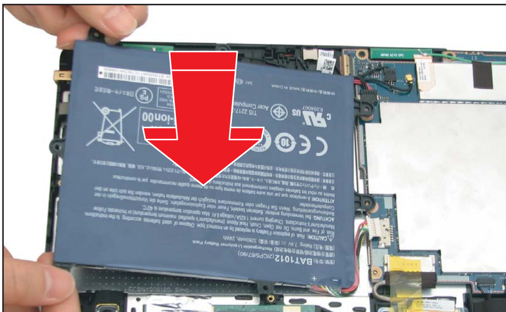
Figure 5-31. Installing the Battery
