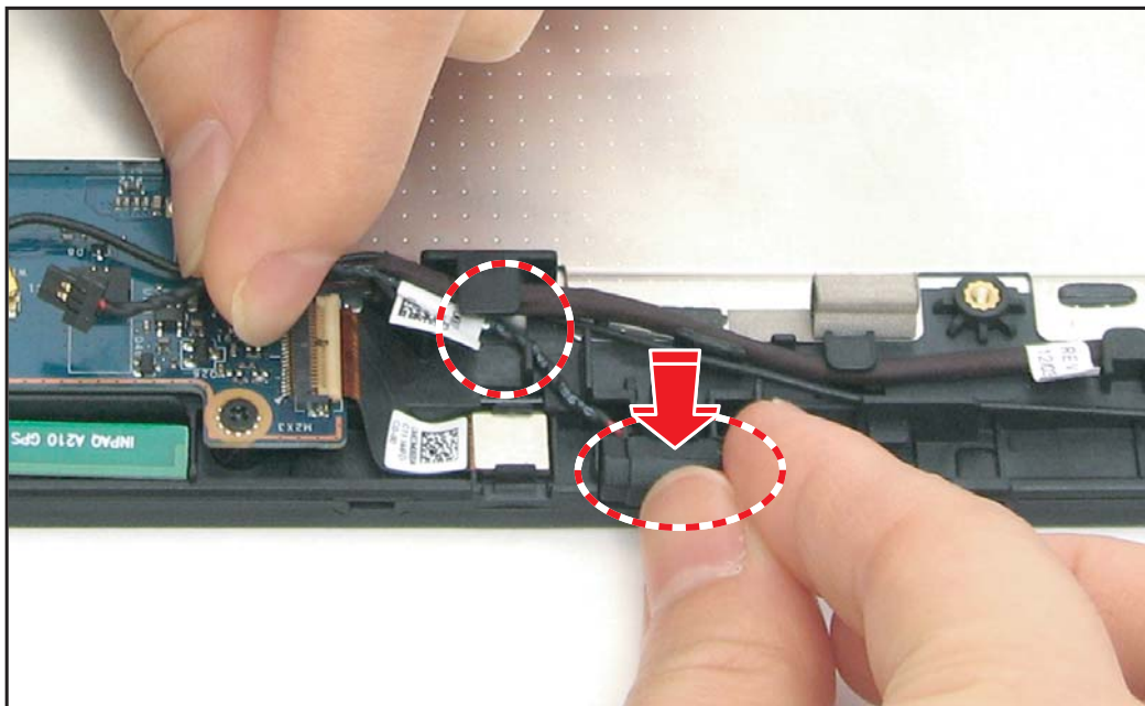
Figure 5-63. Installing the Microphone
