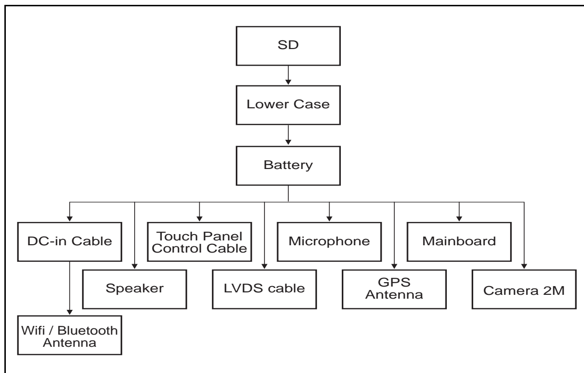
Figure 5-1. Maintenance Flow
