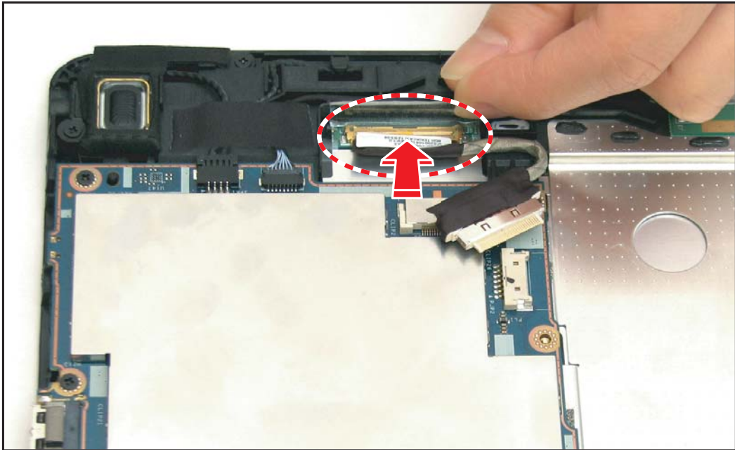
Figure 5-58. Connecting the LVDS Cable (1 of 2)
