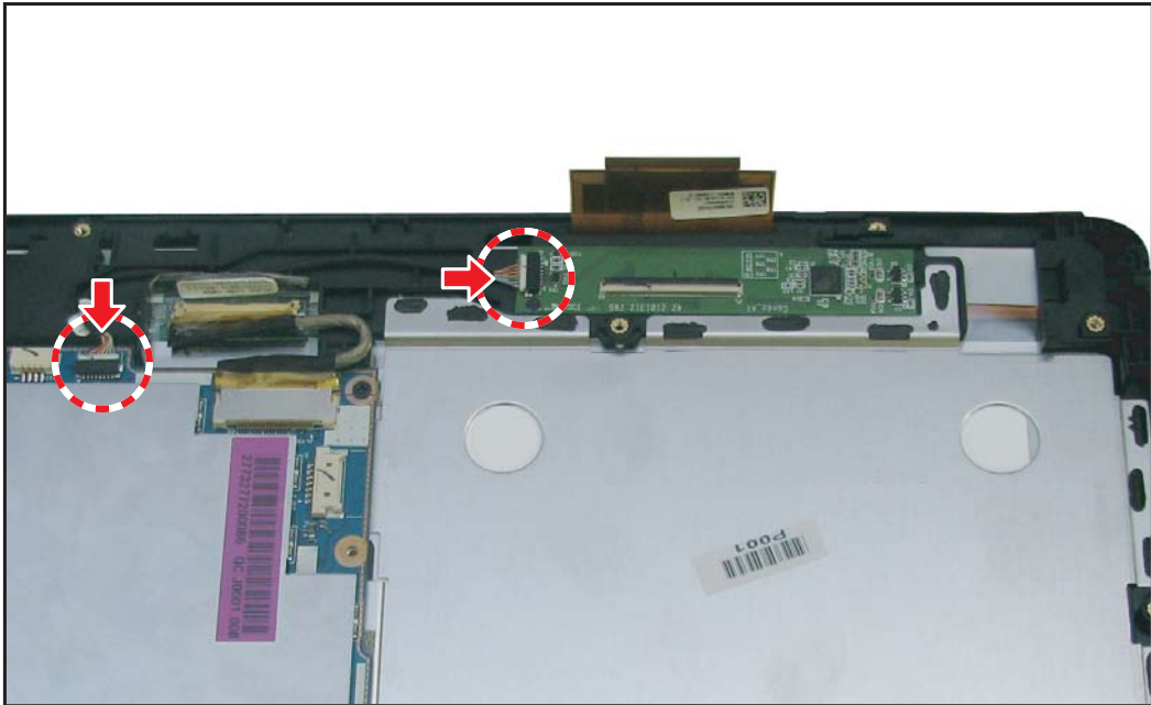
Figure 5-52. Connecting the Touch Panel Control Cable Connectors
