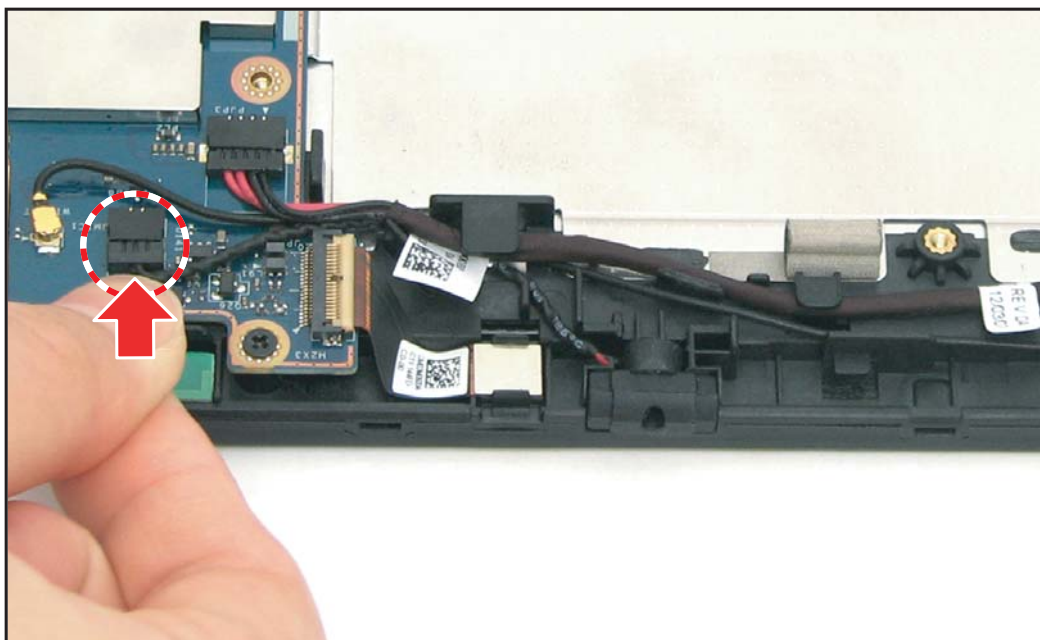
Figure 5-64. Connecting the Microphone Cable Connector
